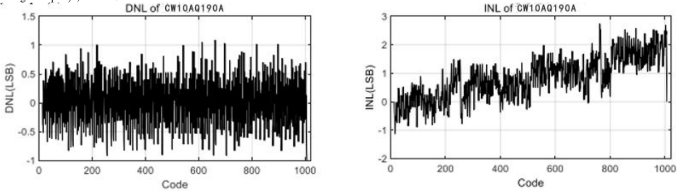
picture8.1 CW10AQ190A linear error test curve
