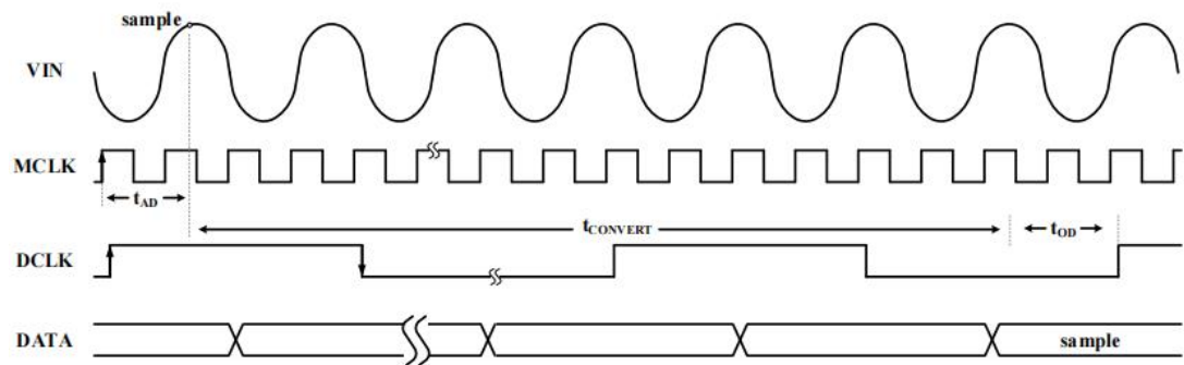
picture 11.10 DCLK Generate Timing
