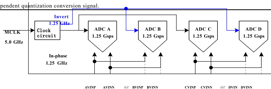
picture5.3 Dual-channel interleaved working mode
